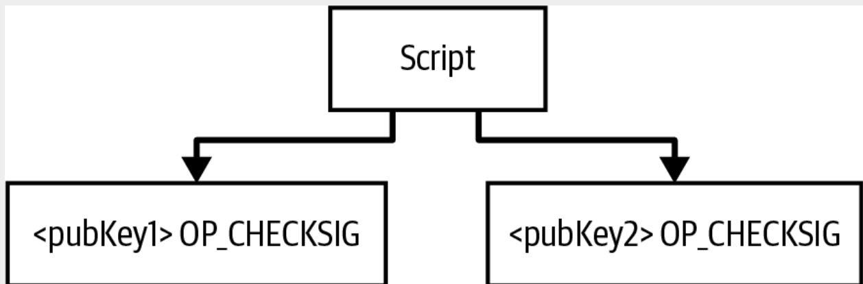
Figure 45. An alternative script tree.
