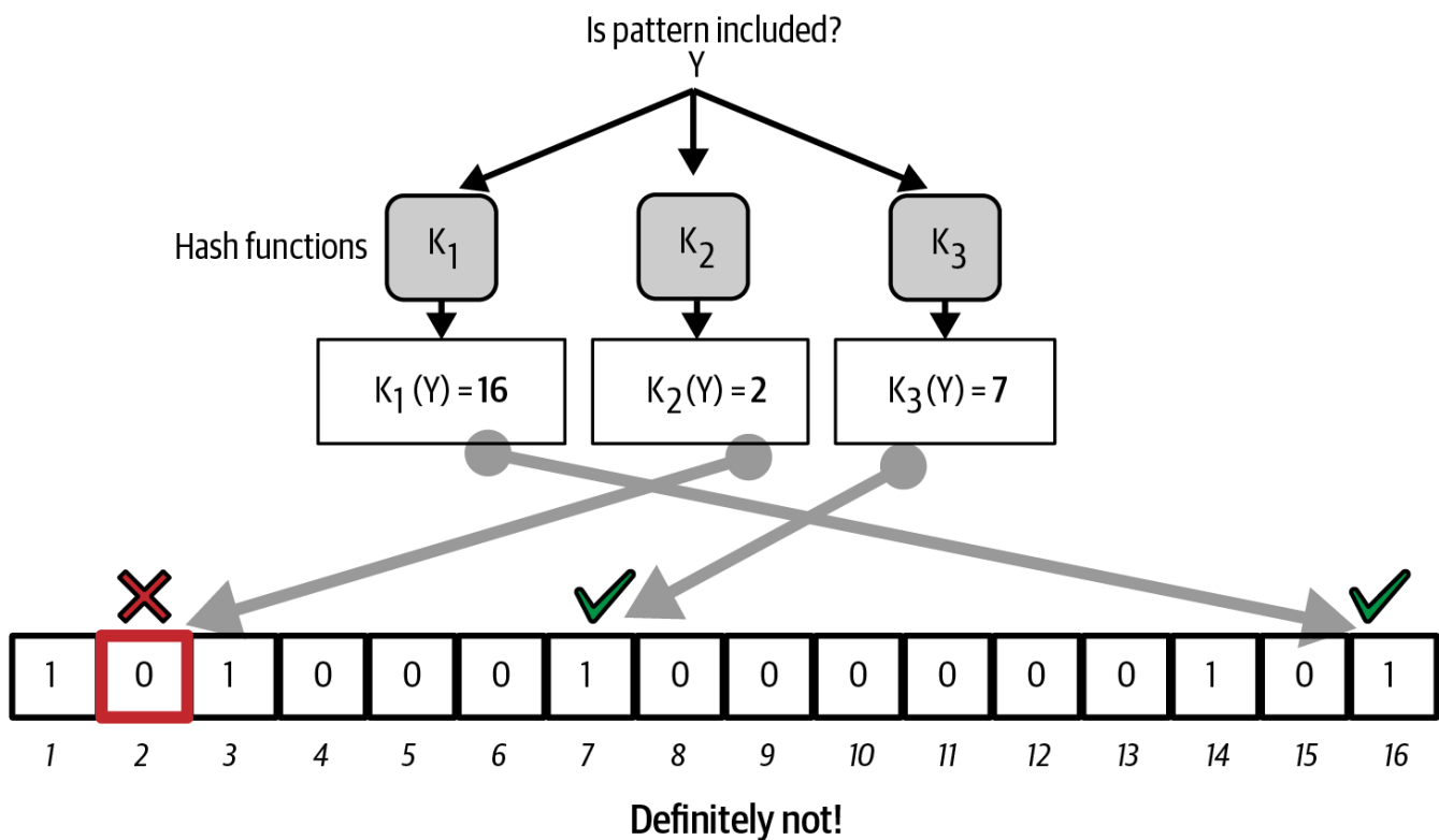
Figure 56. Testing the existence of pattern "Y" in the bloom filter. The result is a definitive negative match, meaning "Definitely Not!"
