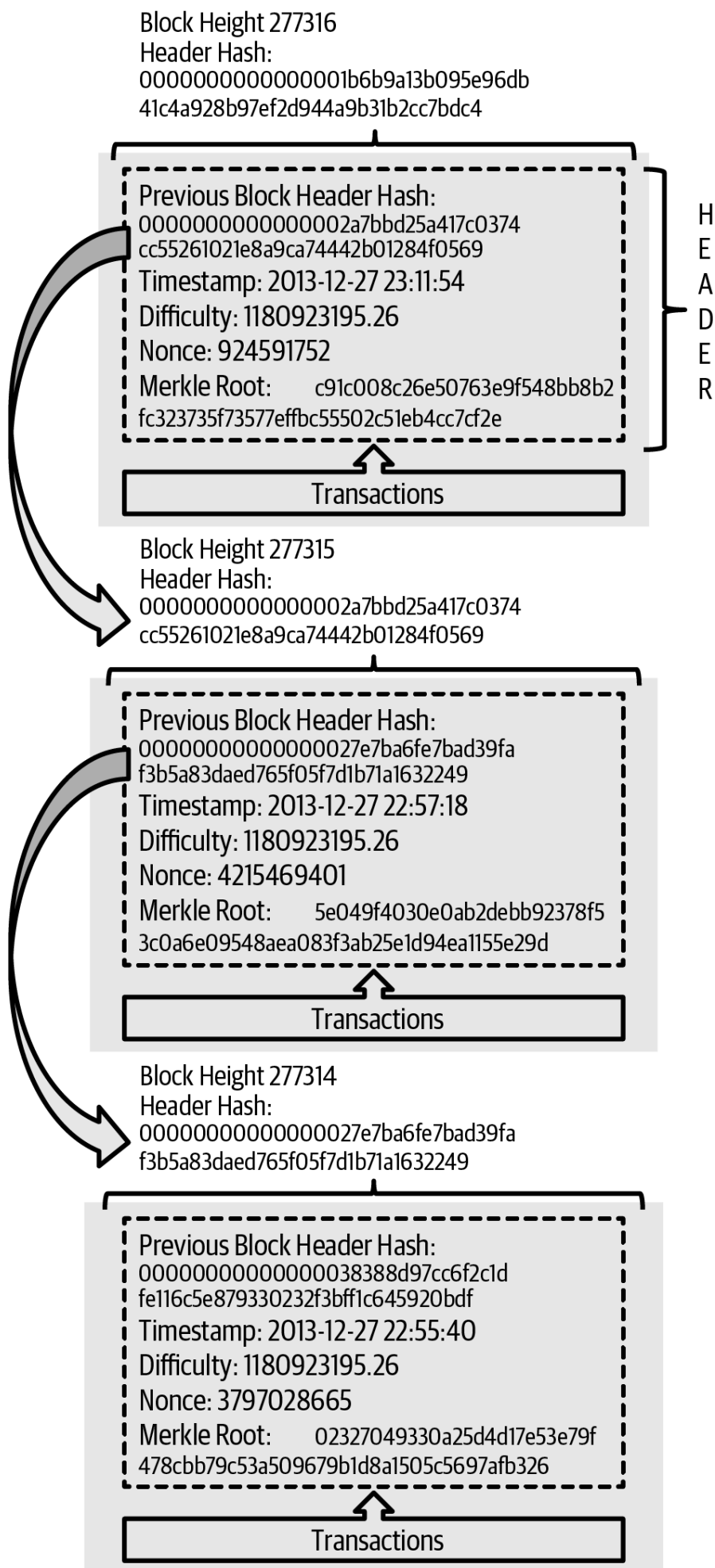
Figure 57. Blocks linked in a chain by each referencing the previous block header hash.
