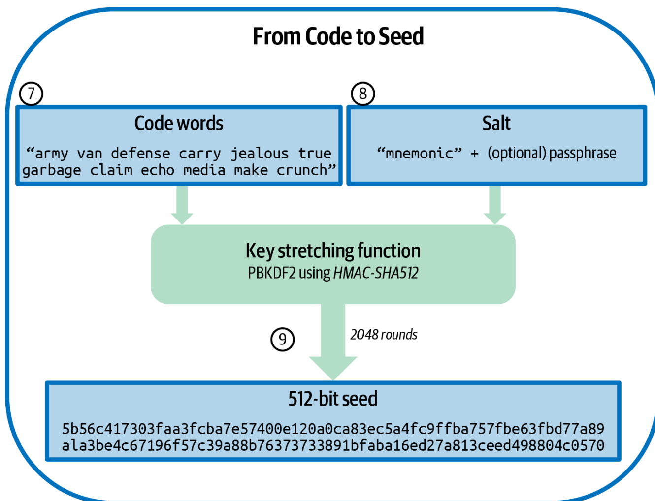
Figure 26. From recovery code to seed.
