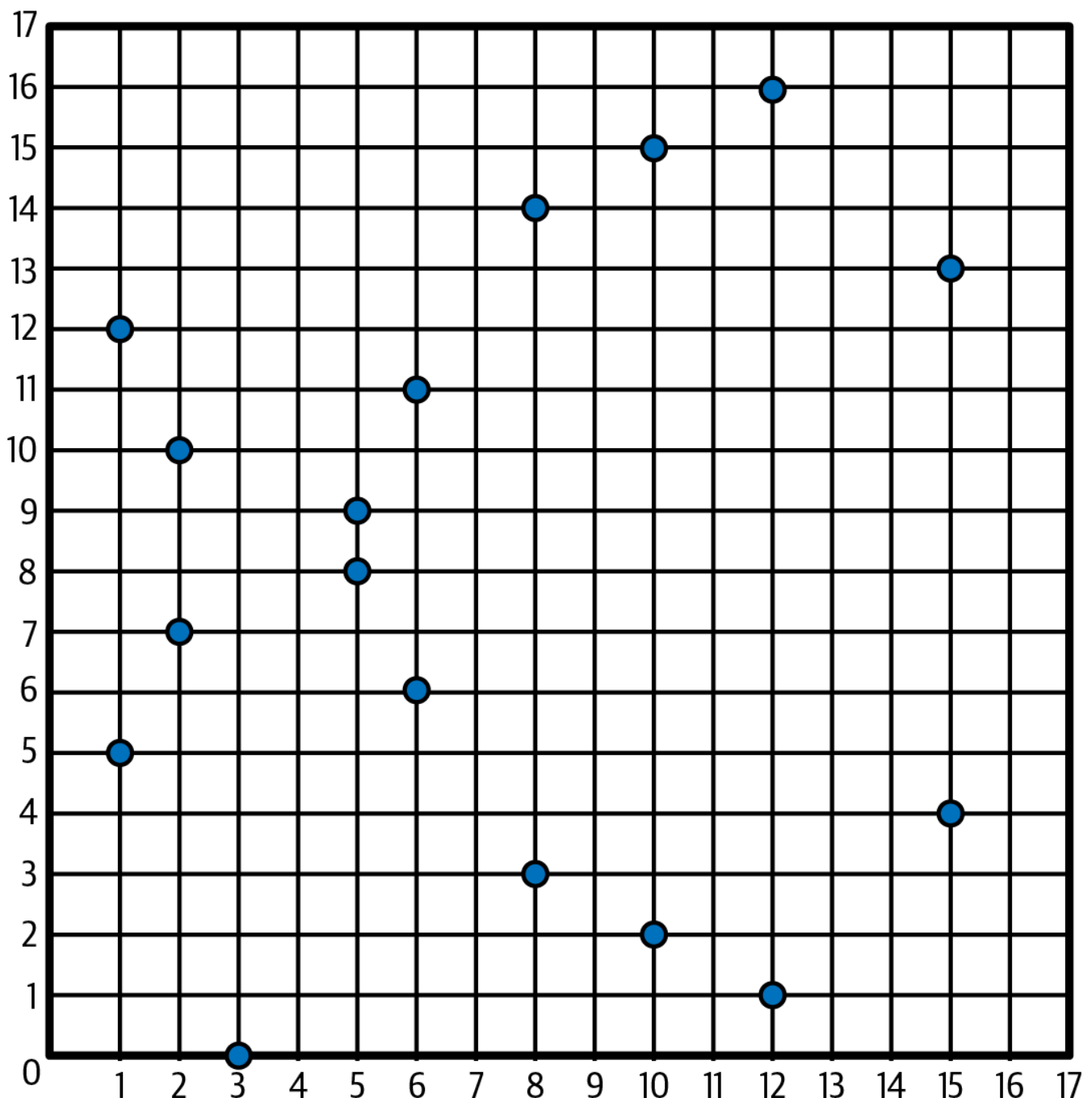
Figure 14. Elliptic curve cryptography: visualizing an elliptic curve over \mathbb{F}(p) , with p=17 .
