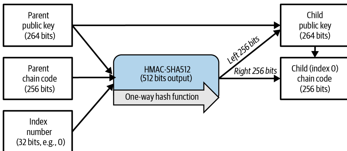
Figure 29. Extending a parent public key to create a child public key.
