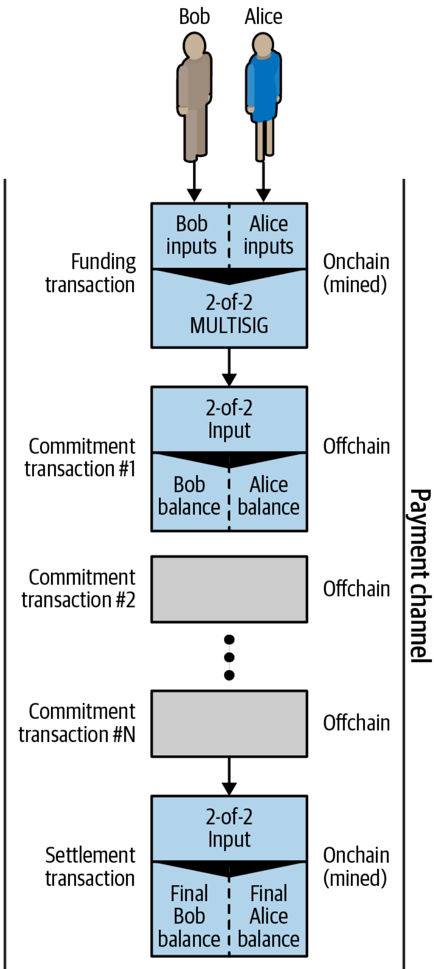
Figure 66. A payment channel between Bob and Alice, showing the funding, commitment, and settlement transactions.
