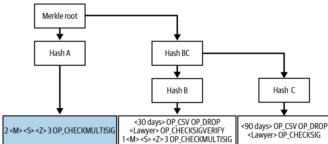
Figure 43. A MAST with the most-expected script in the best position.
