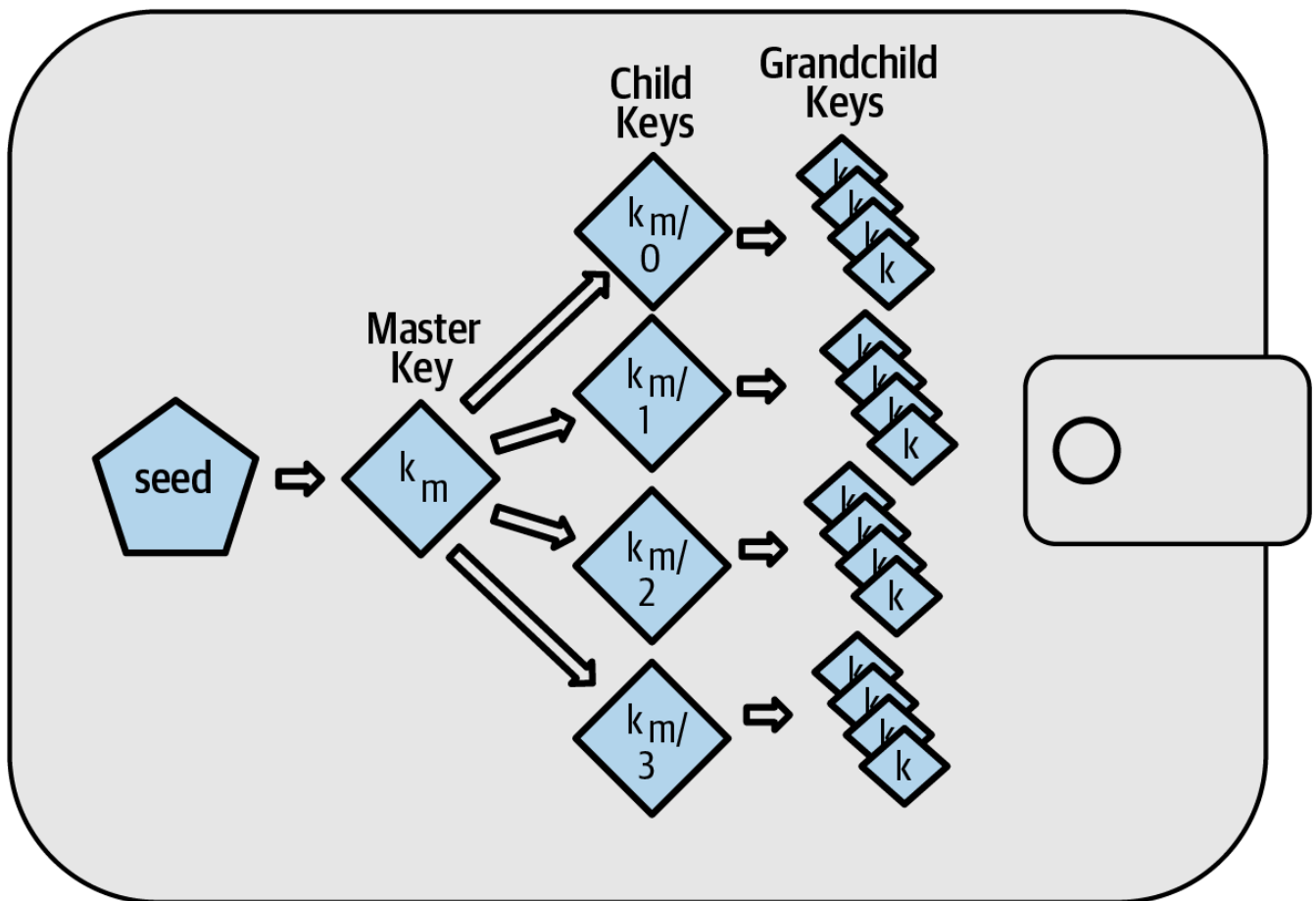
Figure 24. HD wallet: a tree of keys generated from a single seed.
