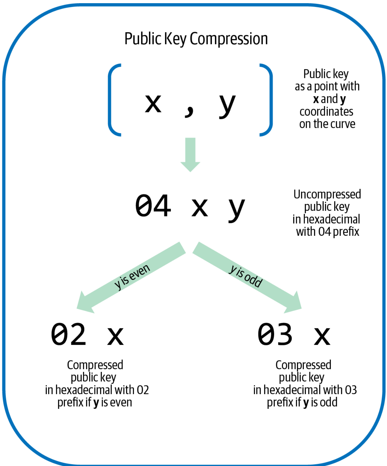
Figure 19. Public key compression.
