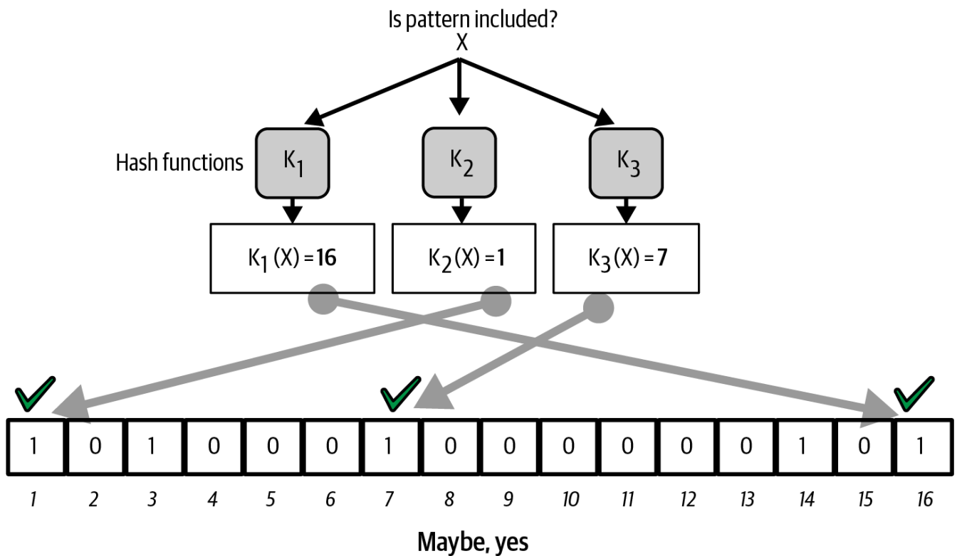
Figure 55. Testing the existence of pattern "X" in the bloom filter. The result is a probabilistic positive match, meaning "Maybe."
