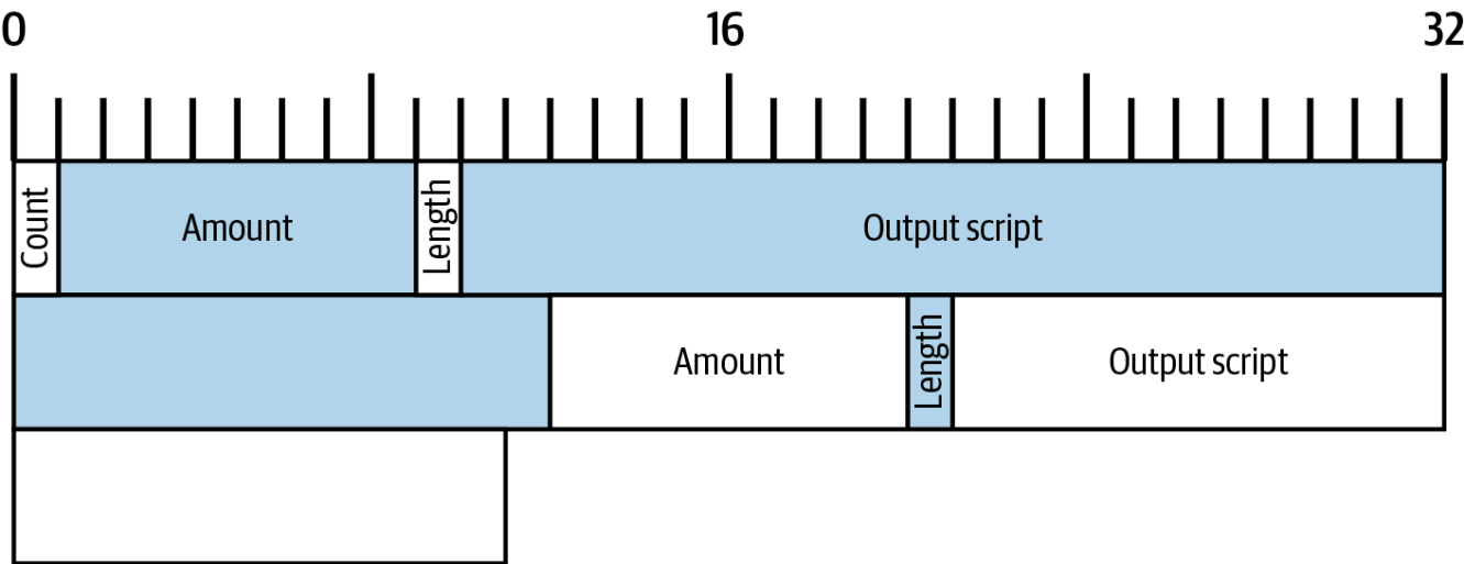
Figure 34. A byte map of the outputs field from Alice's transaction.
