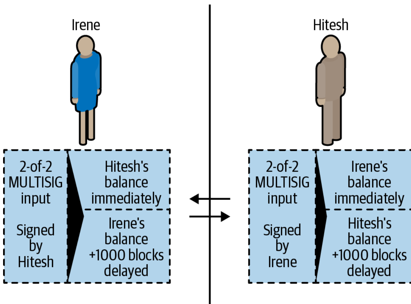
Figure 70. Two asymmetric commitment transactions with delayed payment for the party holding the transaction.
