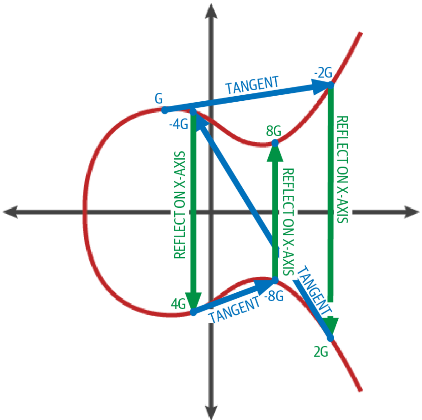
Figure 15. Elliptic curve cryptography: visualizing the multiplication of a point G by an integer k on an elliptic curve.
