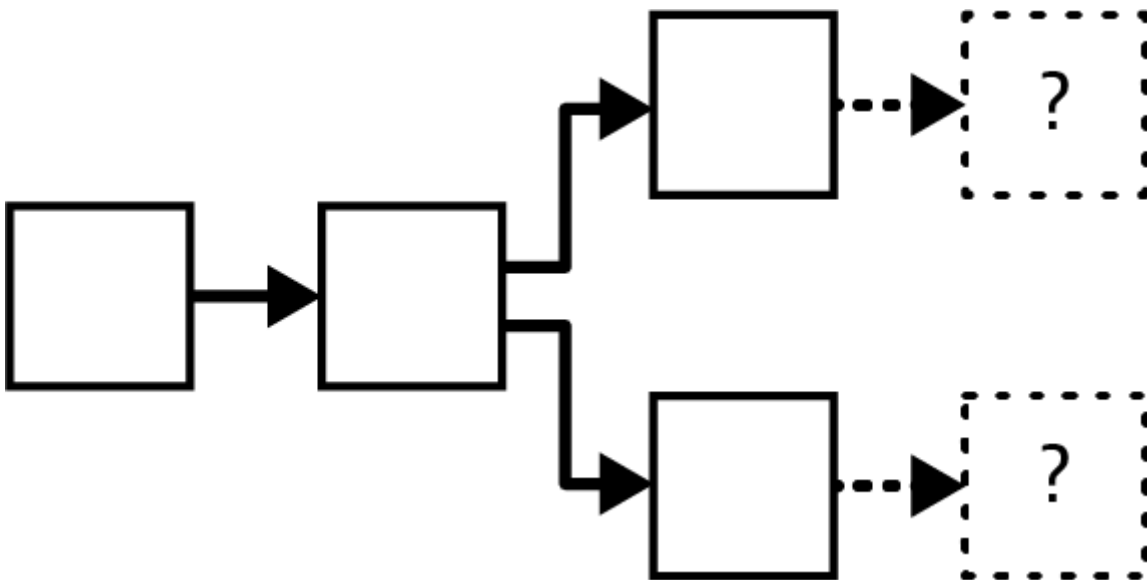
Figure 47. A blockchain fork requiring a mining race.
