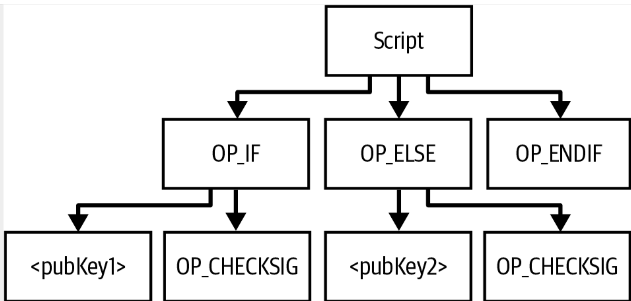
Figure 44. An abstract syntax tree (AST) for a script.
