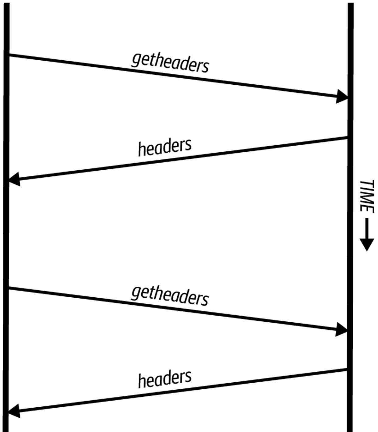
Figure 51. Lightweight client synchronizing the block headers.
