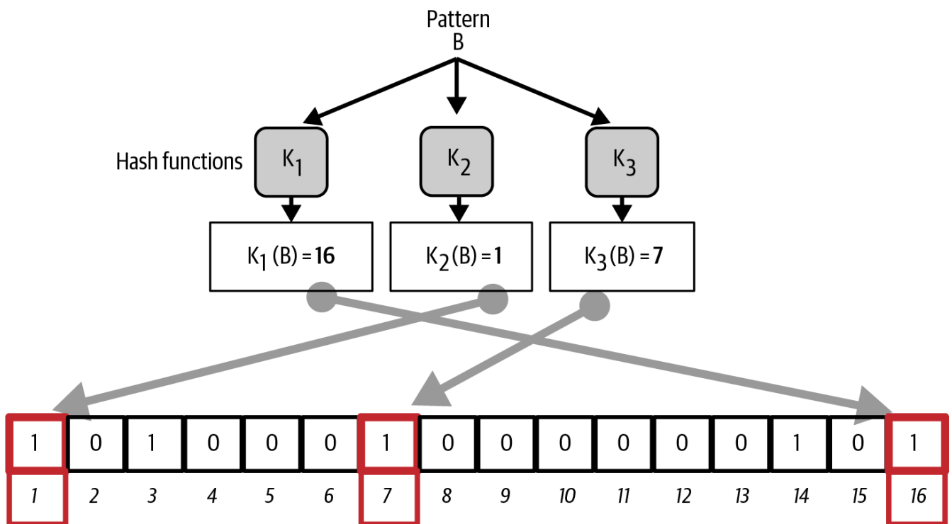
Figure 54. Adding a second pattern "B" to our simple bloom filter.
