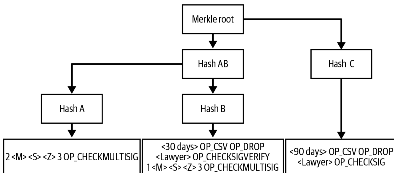
Figure 41. A MAST with three subscripts.
