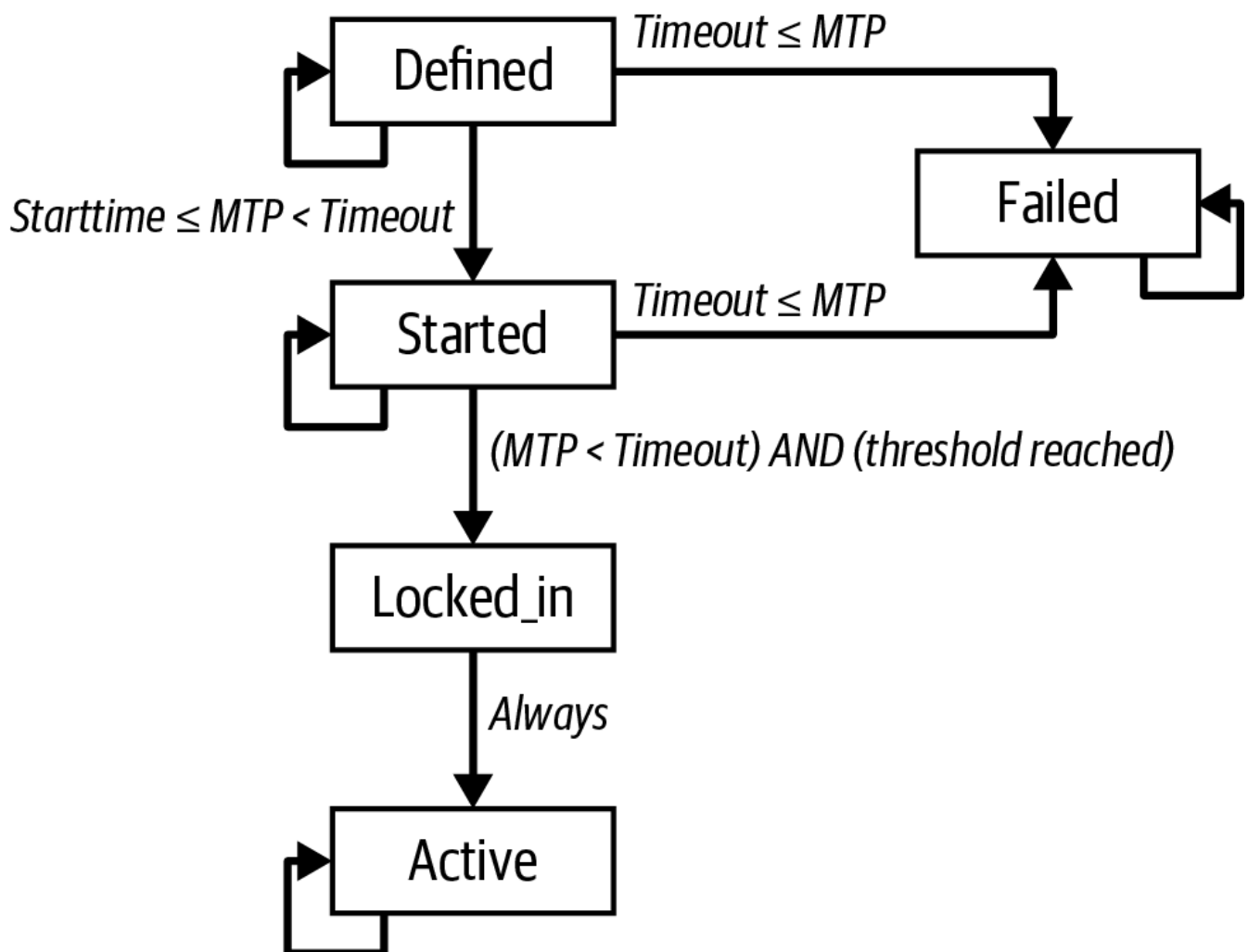
Figure 65. BIP9 state transition diagram.
