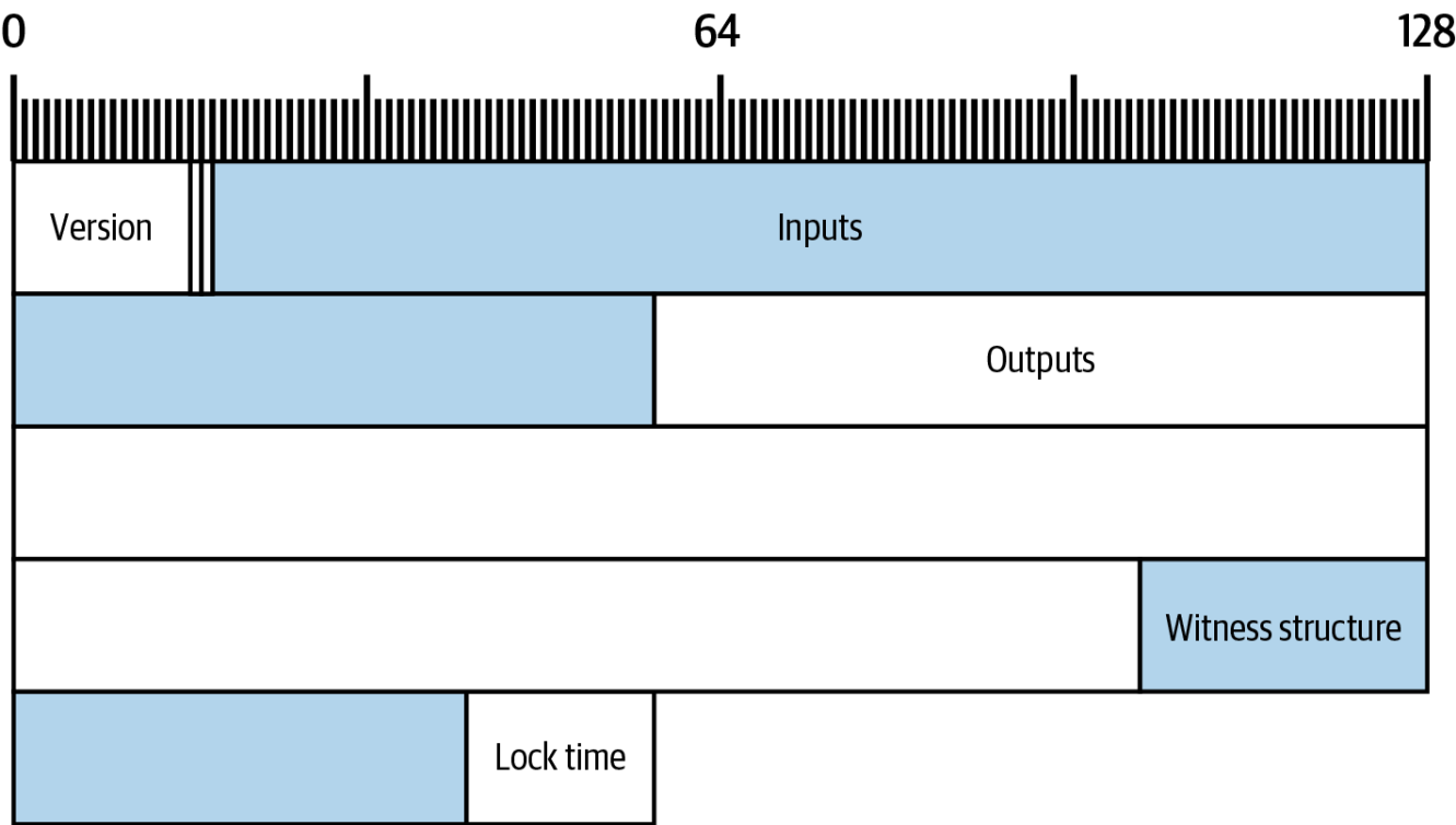
Figure 36. A byte map of Alice’s transaction.
