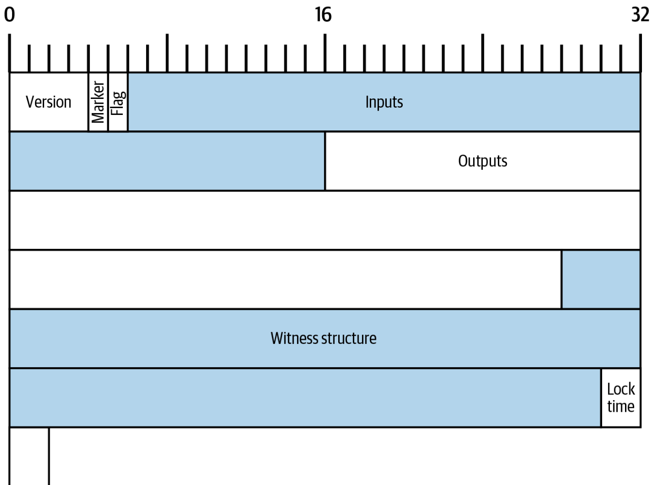
Figure 31. A byte map of Alice's transaction.
