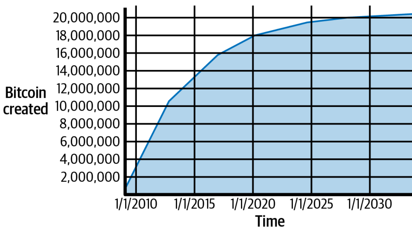
Figure 63. Supply of bitcoin currency over time based on a geometrically decreasing issuance rate.
