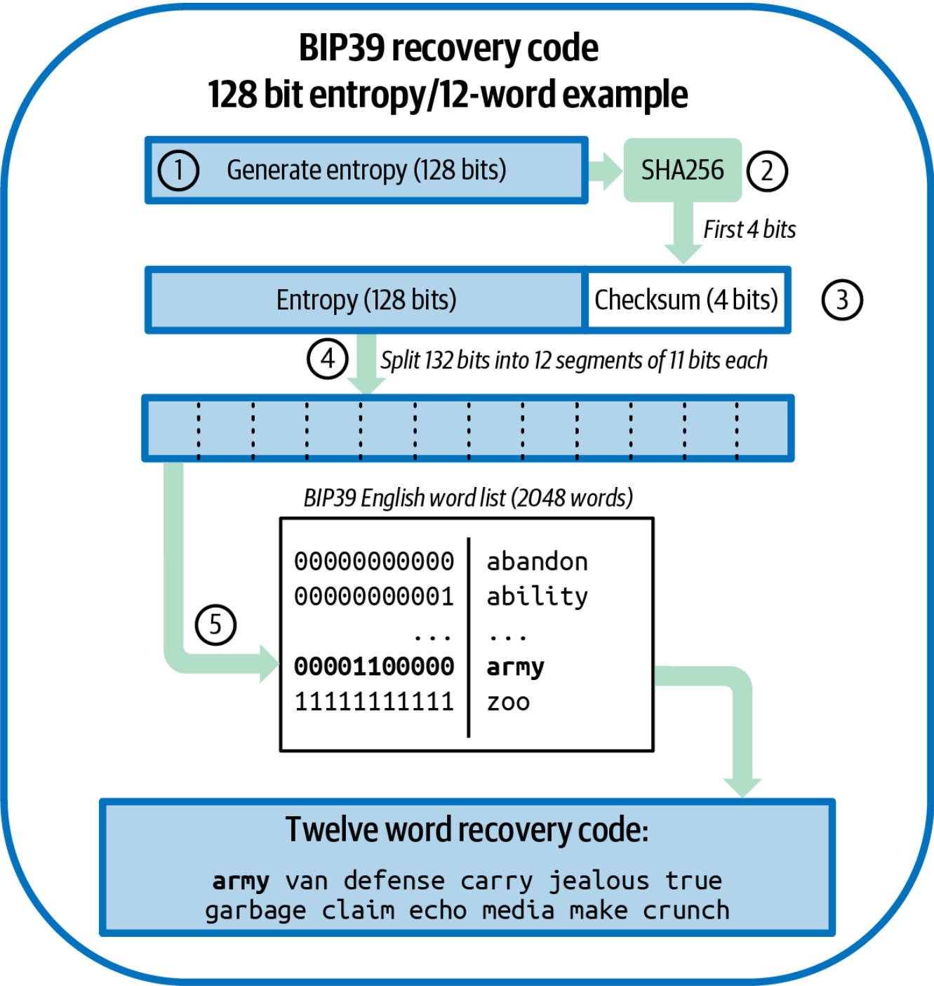
Figure 25. Generating entropy and encoding as a recovery code.
