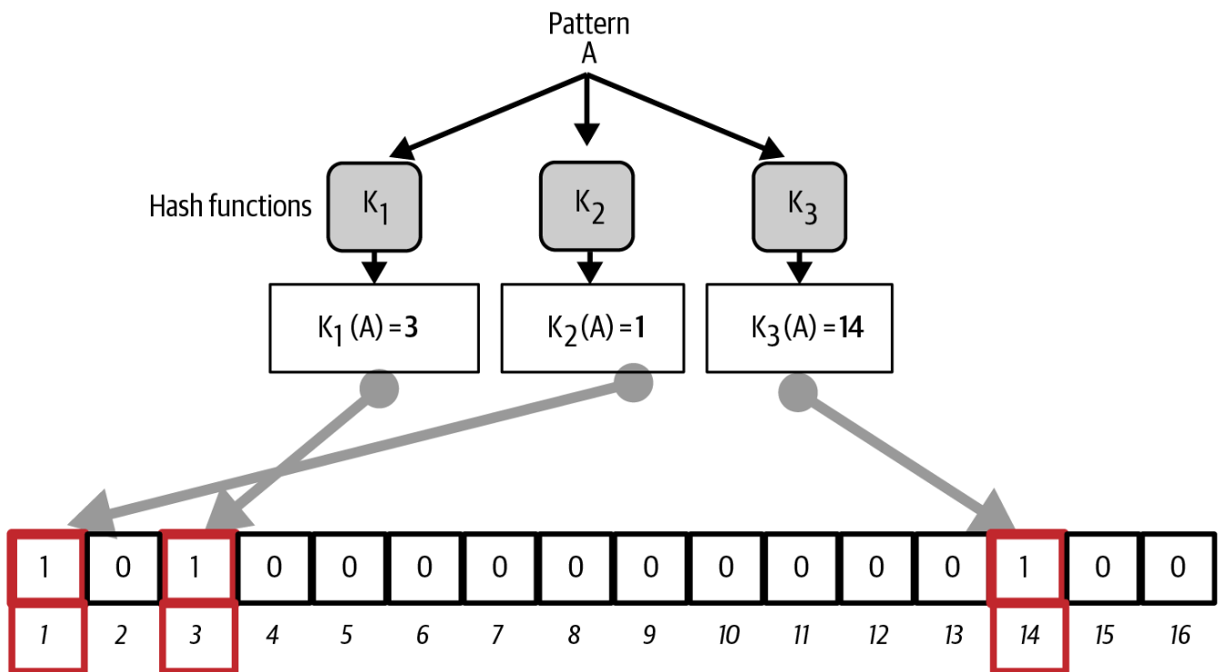
Figure 53. Adding a pattern "A" to our simple bloom filter.
