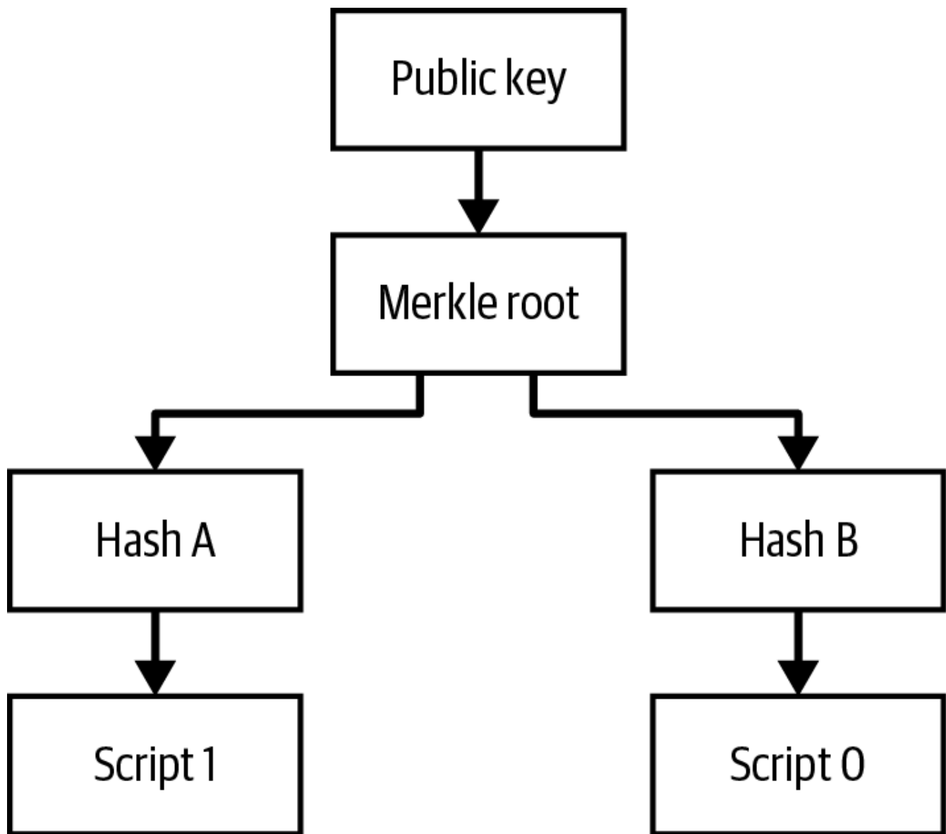
Figure 46. A taproot with the public key committing to a merkle root.
