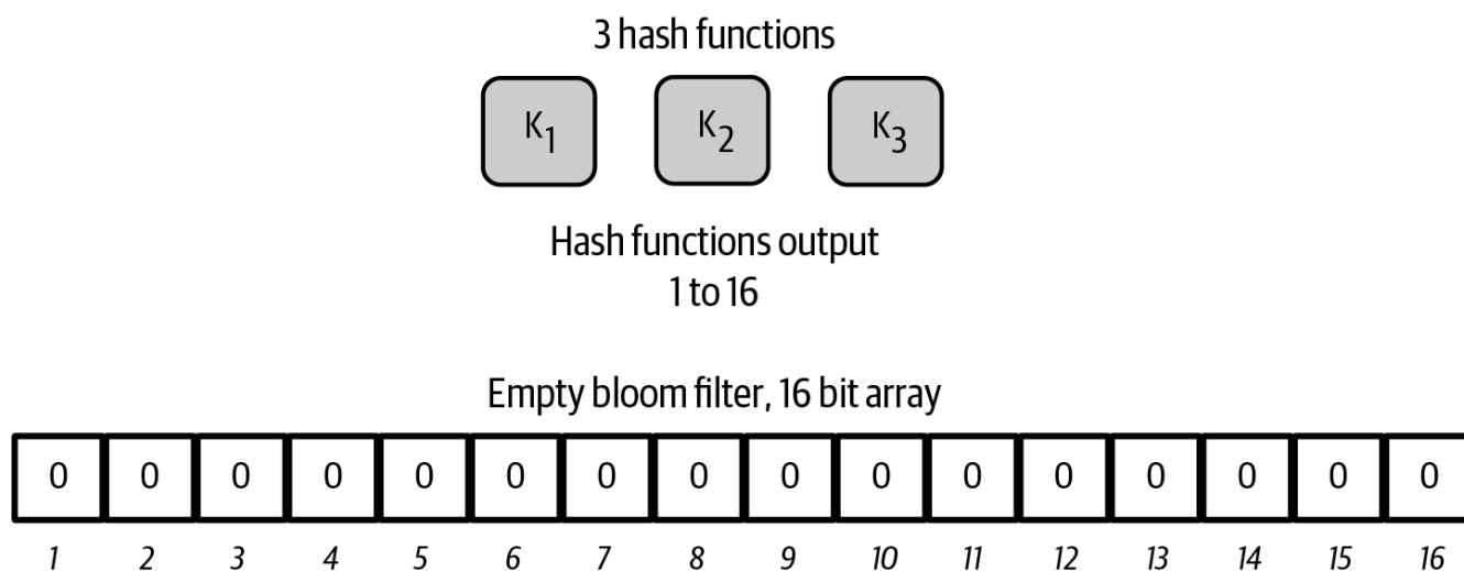
Figure 52. An example of a simplistic bloom filter, with a 16-bit field and three hash functions.
