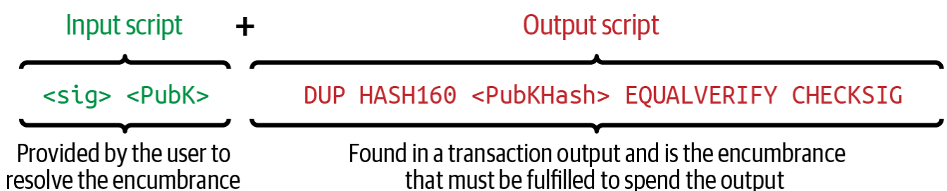
Figure 37. Combining input and output scripts to evaluate a transaction script.
