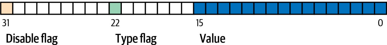
Figure 33. BIP68 definition of sequence encoding (Source: BIP68).
