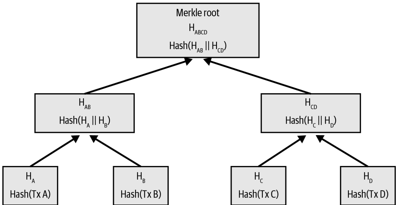
Figure 58. Calculating the nodes in a merkle tree.
