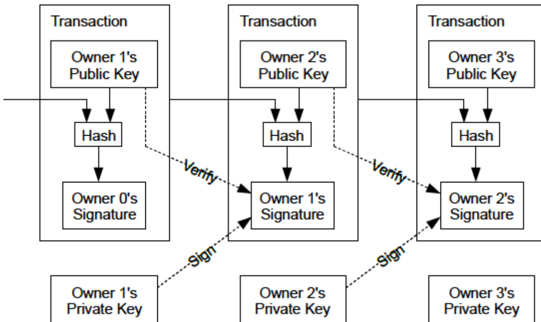
Figure 12. Transaction chain from original Bitcoin paper.
