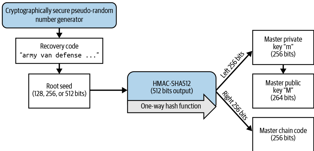
Figure 27. Creating master keys and chain code from a root seed.
