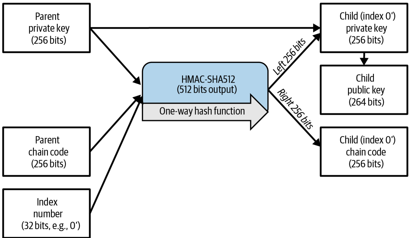
Figure 30. Hardened derivation of a child key; omits the parent public key.
