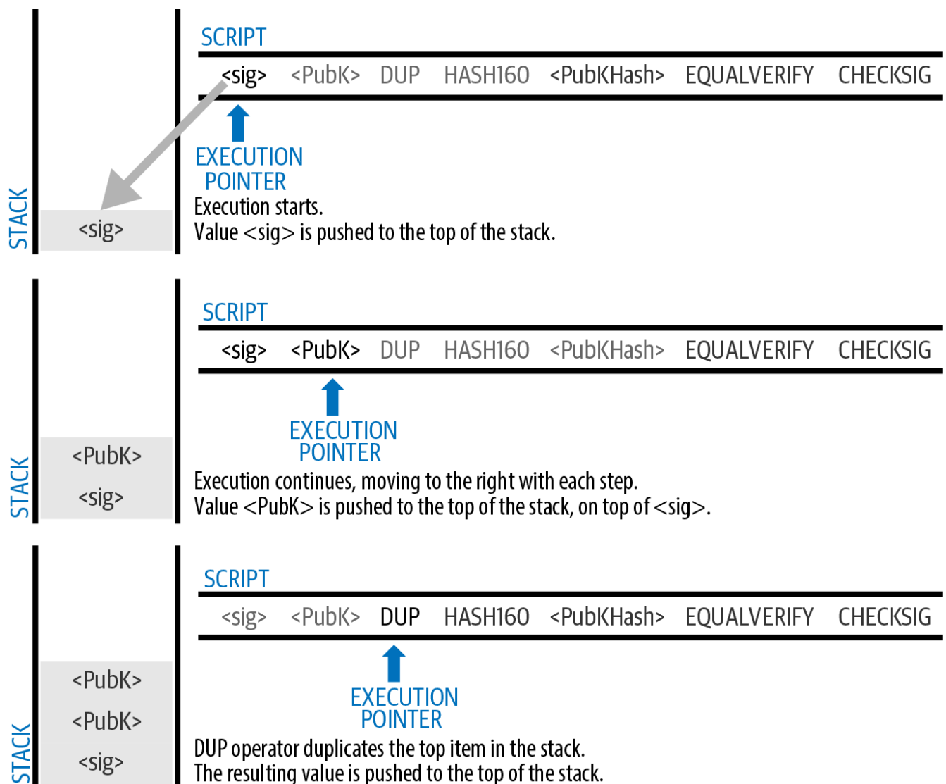
Figure 39. Evaluating a script for a P2PKH transaction (part 1 of 2).
