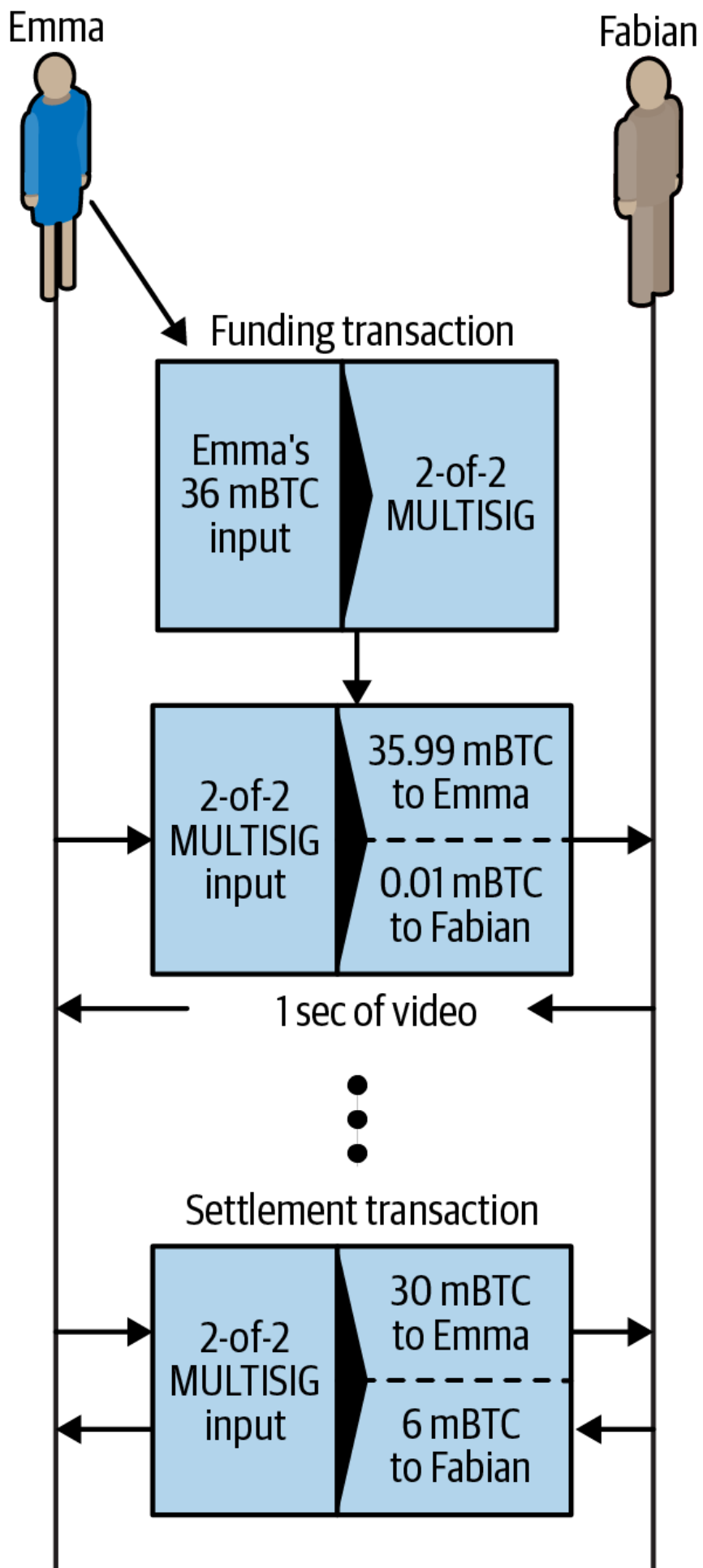
Figure 68. Emma's payment channel with Fabian, showing the commitment transactions that update the balance of the channel.
