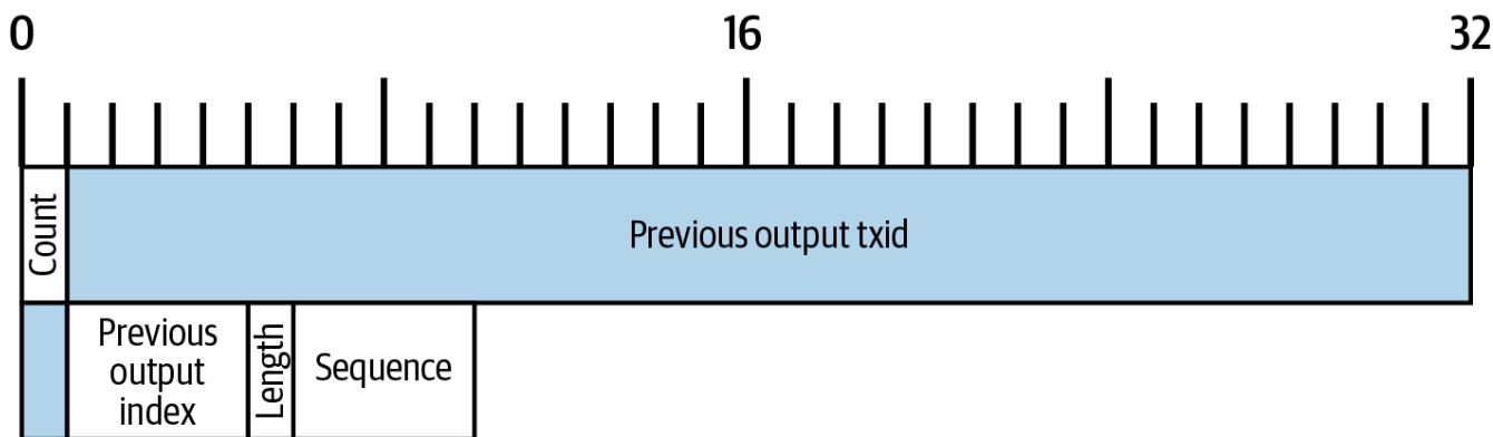
Figure 32. Map of bytes in the inputs field of Alice's transaction.
