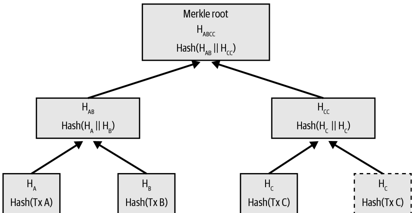
Figure 59. Duplicating one data element achieves an even number of data elements.
