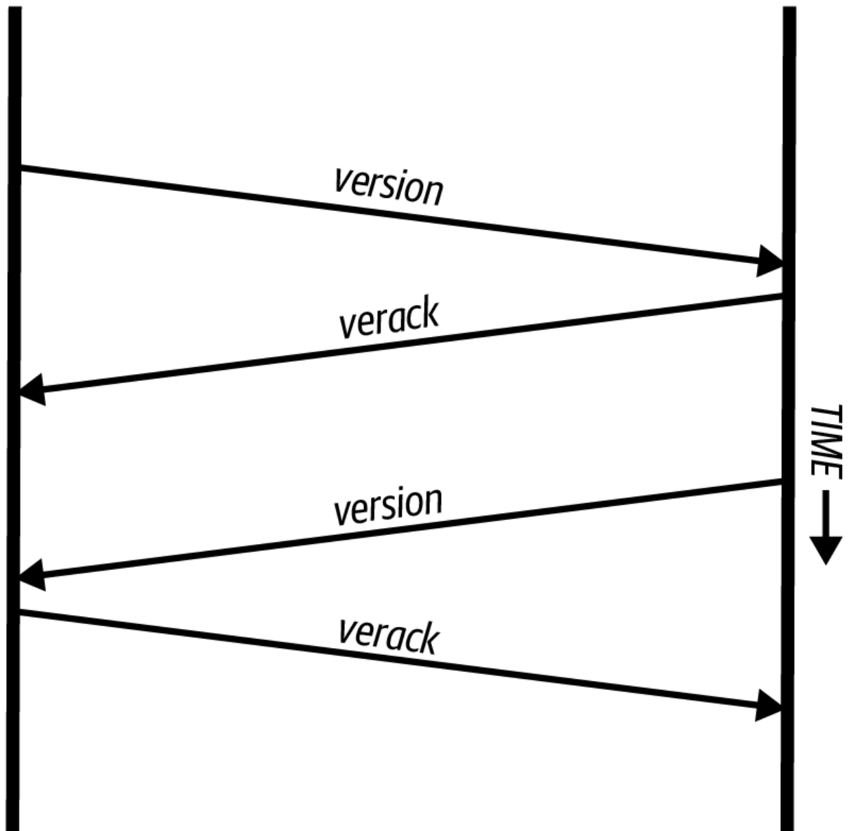
Figure 49. The initial handshake between peers.
