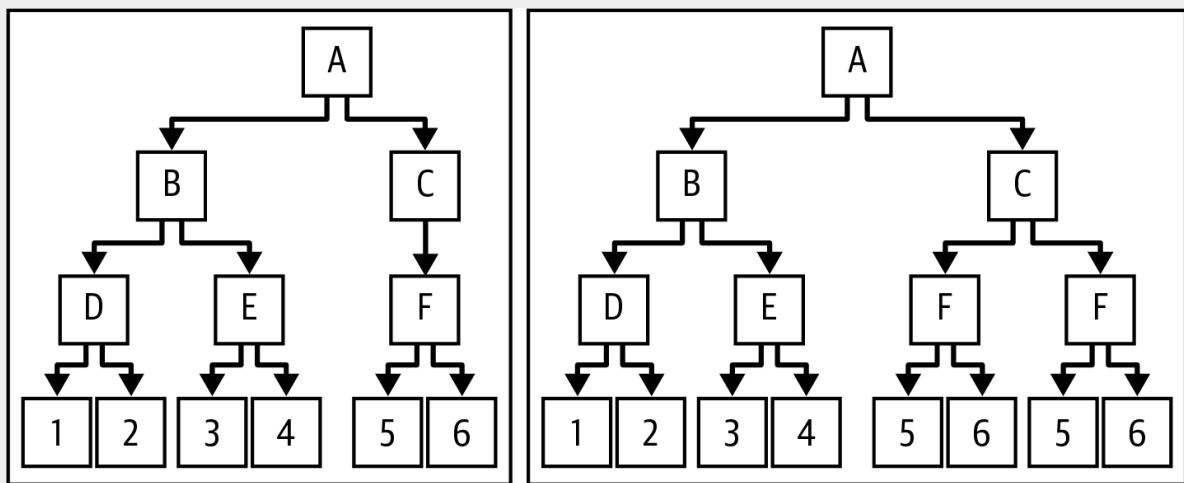
Figure 60. Two Bitcoin-style merkle trees with the same root but a different number of leaves.
