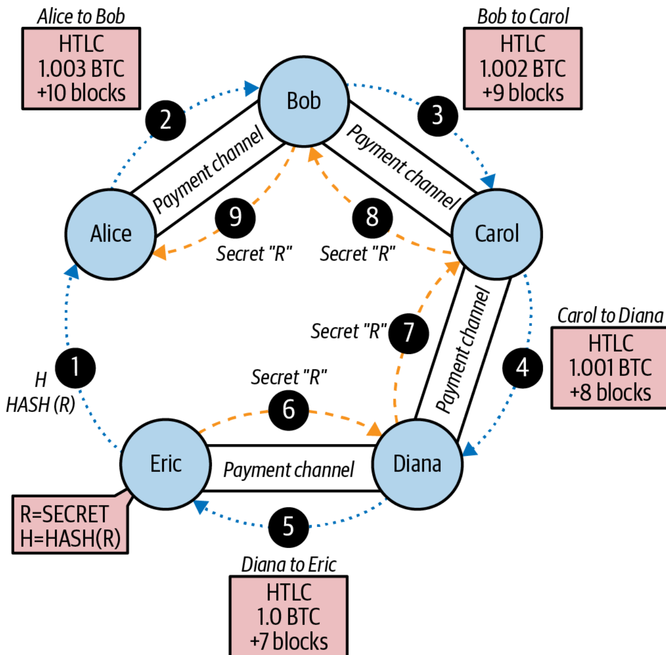
Figure 72. Step-by-step payment routing through an LN.
