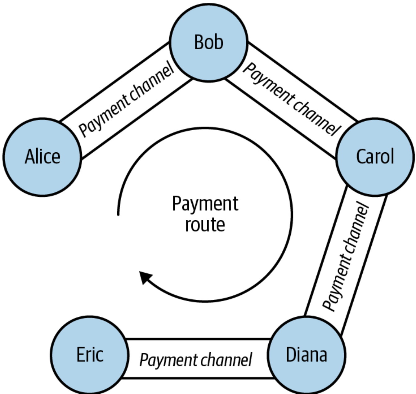
Figure 71. A series of bidirectional payment channels linked to form an LN that can route a payment from Alice to Eric.
