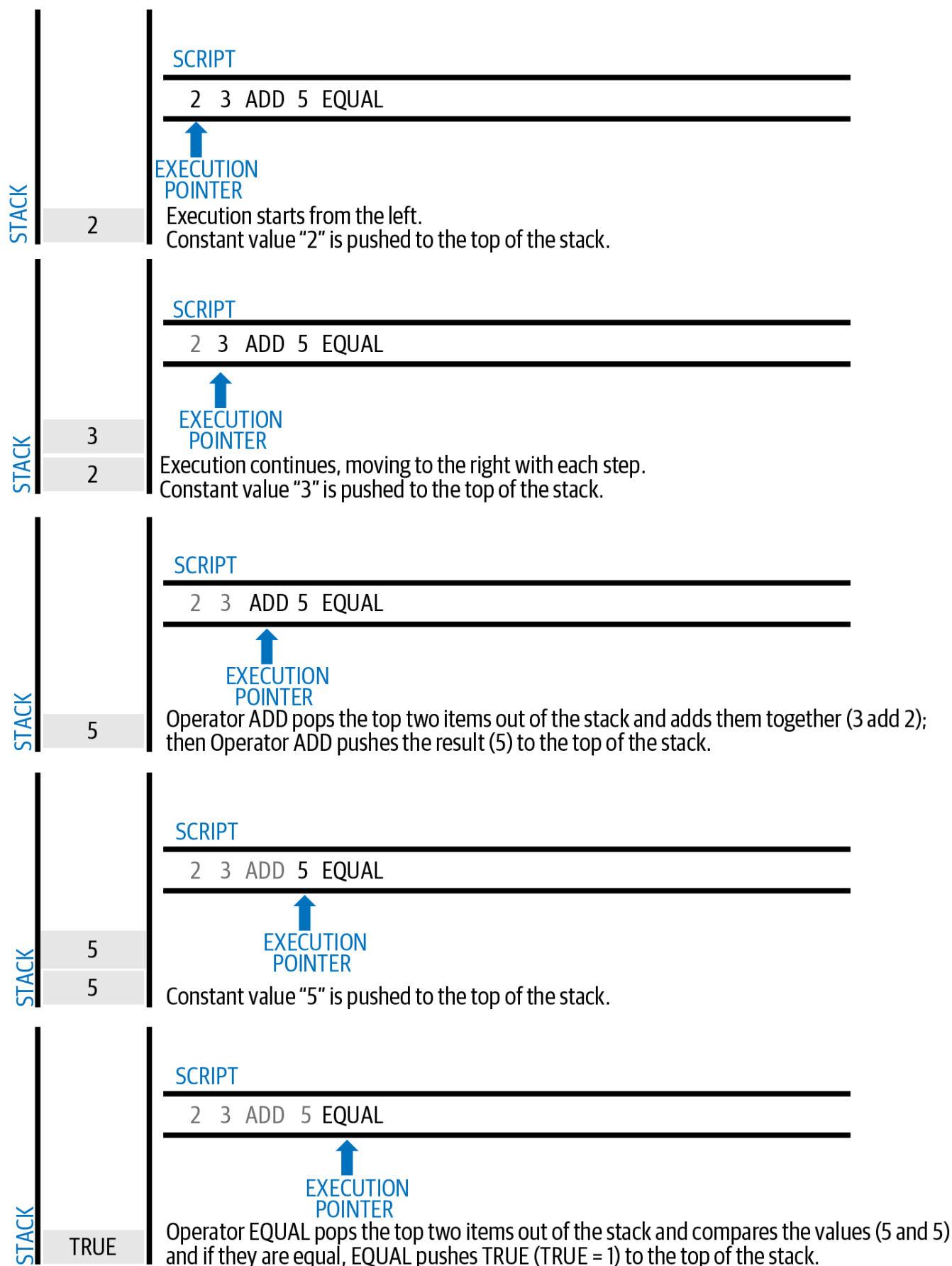
Figure 38. Bitcoin's script validation doing simple math.
