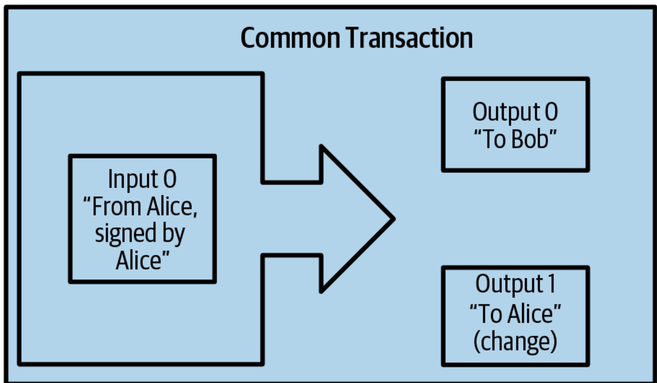
Figure 6. Most common transaction.
