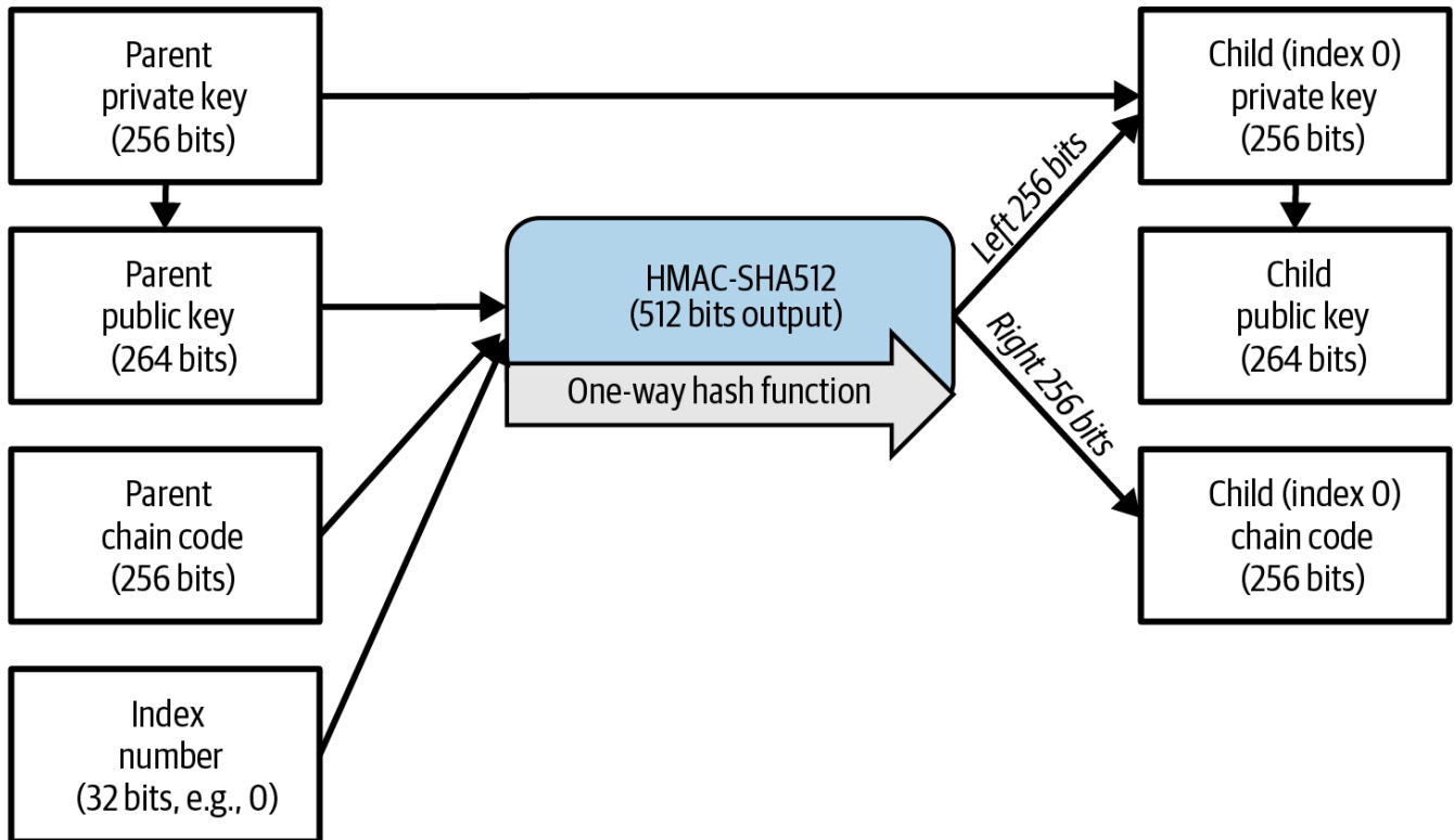
Figure 28. Extending a parent private key to create a child private key.
