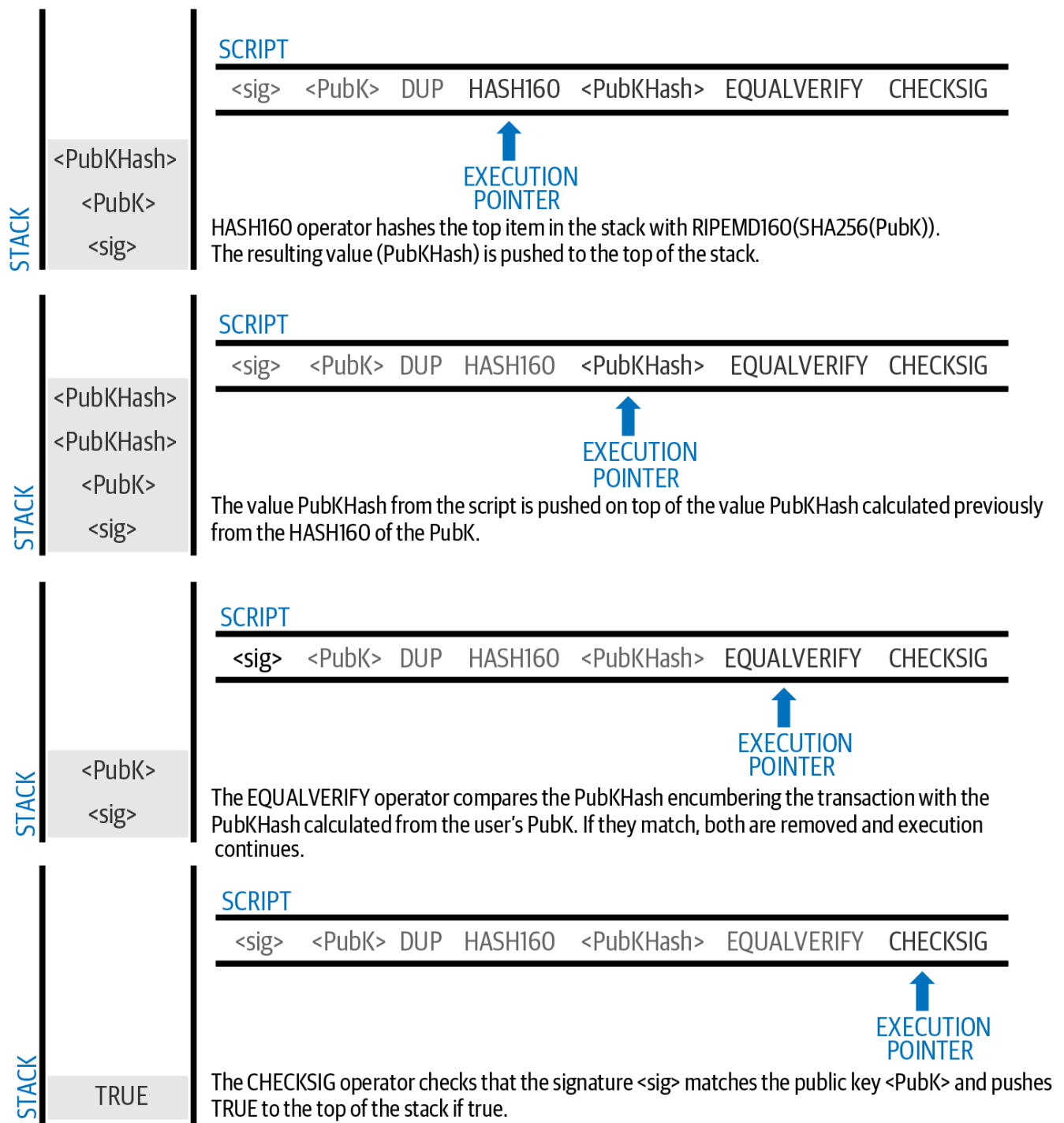
Figure 40. Evaluating a script for a P2PKH transaction (part 2 of 2).
