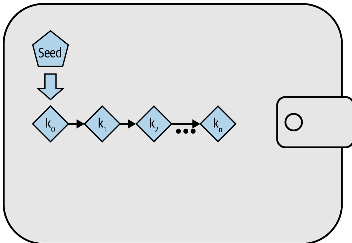
Figure 23. Deterministic key generation: a deterministic sequence of keys derived from a seed for a wallet database.
