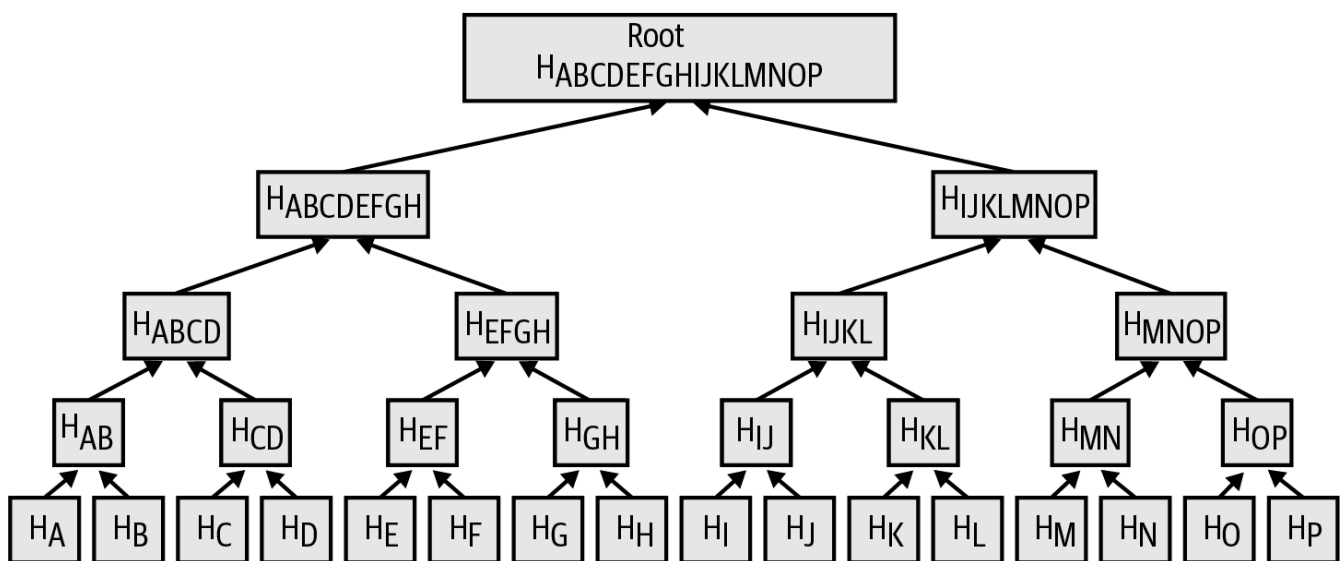
Figure 61. A merkle tree summarizing many data elements.
